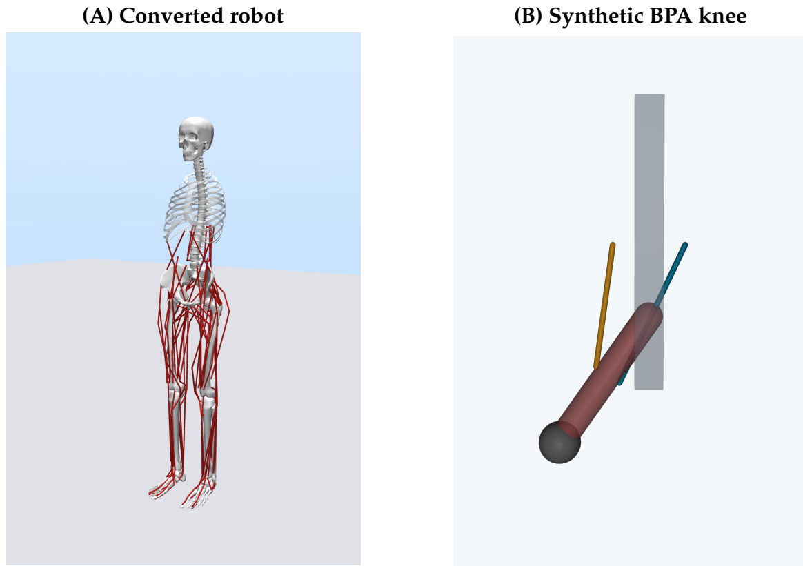
Figure 3.10: Native MuJoCo renders of (A) the converted Gait2392 robot at its saved reference pose, with muscle paths visible, and (B) the independent synthetic antagonist-BPA knee at an illustrative static angle of -35^\circ . Cyan and gold identify its named flexor and extensor tendon routes; transparency exposes the routes through the view. The models are not shown to the same scale. These views document model construction, not SNS control of the converted robot or validated torque predictions.
