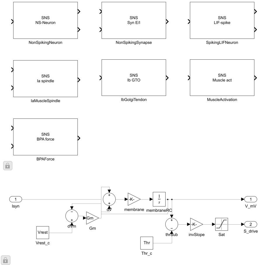
Figure 3.11: Native Simulink diagram exports showing the seven masked library blocks (top) and the internal implementation of the non-spiking neuron (bottom). The library blocks are arranged in a compact display grid for legibility. The BPA force block remains a placeholder. These implementation views do not establish quantitative knee regulation or a completed CAD-coupled Simscape Multibody model.
