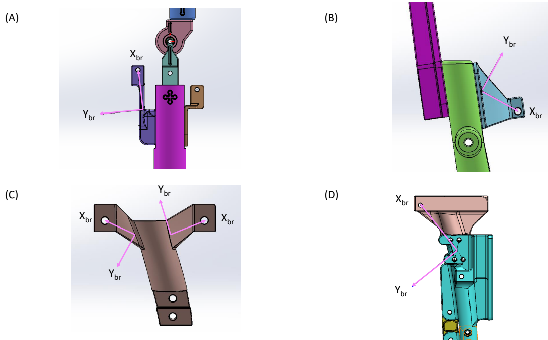
Figure 3.6: Bracket frame orientations for: (A) Flexor configuration on the pinned knee, (B) extensor configuration on the pinned knee, (C) flexor and extensor configurations on the biomimetic knee with \phi 10 mm BPAs, and (D) flexor configuration on the biomimetic knee with the \phi 20 mm BPA.
