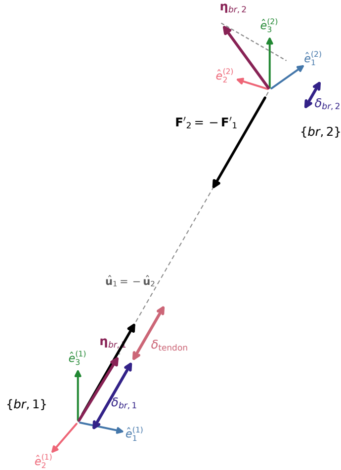
Figure 3.5: Two-bracket displacement and projection along the BPA force path. The force vectors at \{br, 1\} and \{br, 2\} point toward one another and satisfy \mathbf{F}'_2 = -\mathbf{F}'_1 . The bracket projections \delta_{br,1} and \delta_{br,2} are offset from their coordinate frames for clarity, and tendon elongation \delta_{\text{tendon}} continues collinearly from \delta_{br,1} . Colors use a color-vision-deficiency-safe palette and are redundant with labels and line weights.
